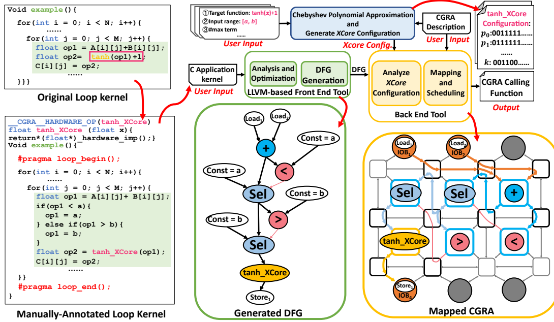
Fig. 6. The software toolchain of LoRA, which can support the custom nonlinear function implementation.
