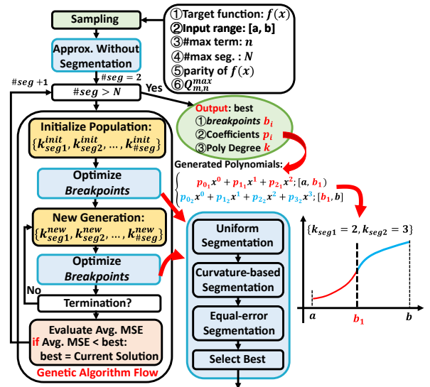
Fig. 3. The proposed Chebyshev-based approximation algorithm flow.
